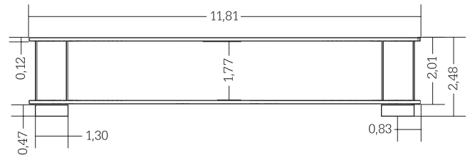
Front view - dimensions in inch*
