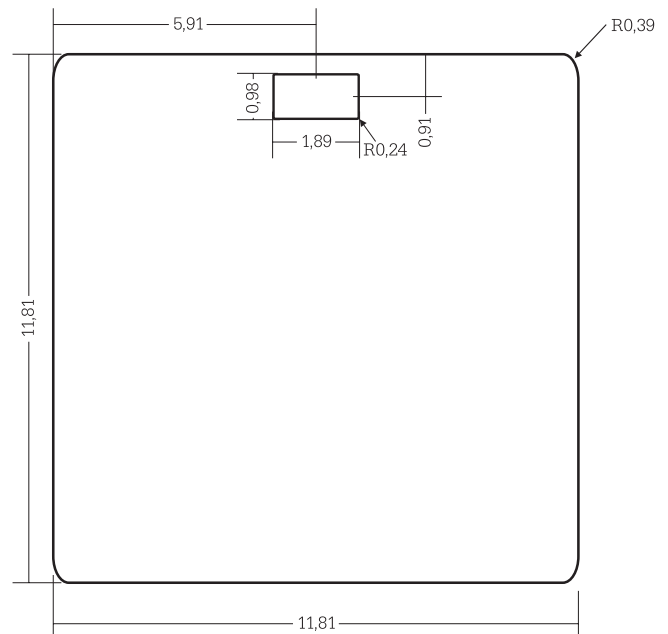
View from top - dimensions in inch*
